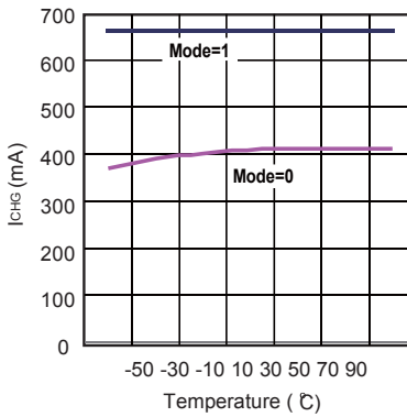
CC Charge Current vs. Temperature
