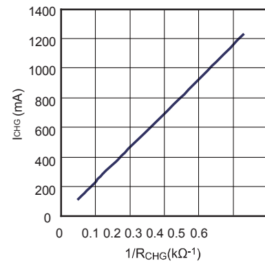
I CHG vs. 1/R CHG
