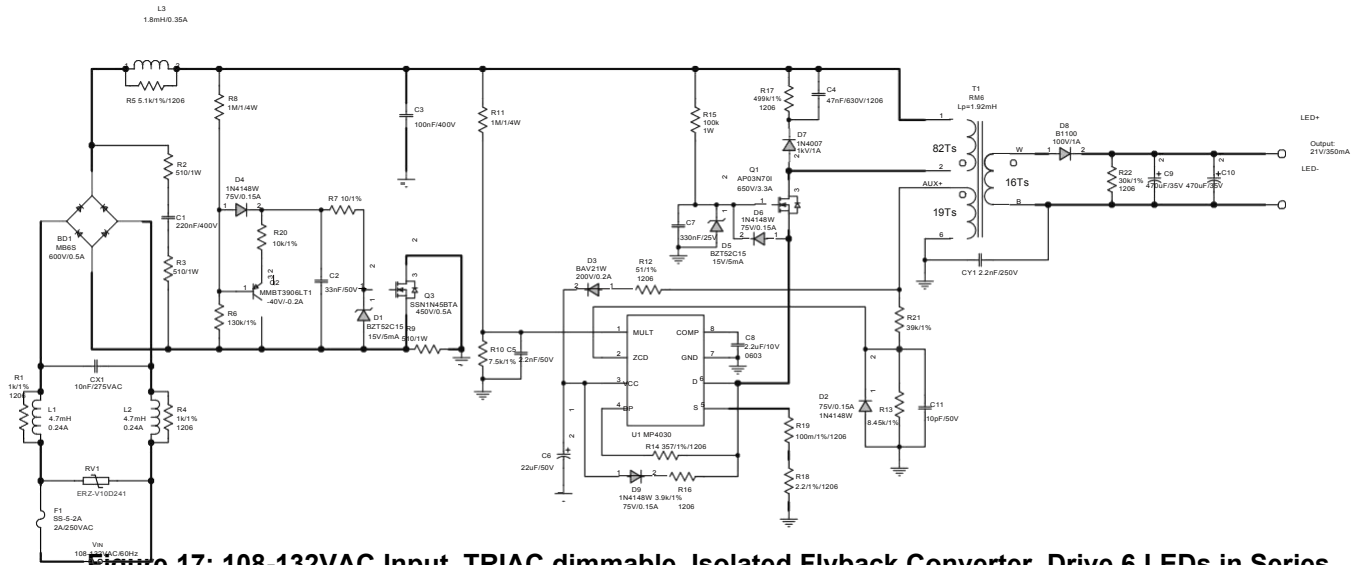
Figure 17: 108-132VAC Input, TRIAC dimmable, Isolated Flyback Converter, Drive 6 LEDs in Series, 350mA LED Current for LED Lighting, EVB Model: EV4030-S-00A
