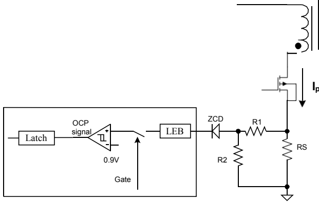
Figure 10: ZCD Over-Current Protection Circuit
