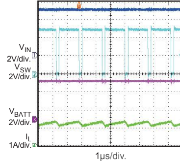
CV Charge Steady State
