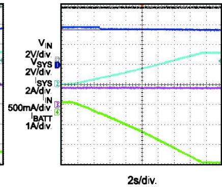
System Current Transient Battery Full, I_{SYS} = 1.2A transient, 0.05A/\mu s
