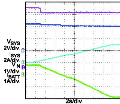
Input Voltage Limit 5V/1A Adapter IN, V_{BATT} = 4.2V Ramp up I_{SYS}
