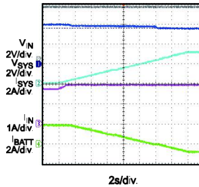
Input Voltage Limit 5V/1A Adapter IN, V_{BATT} = 4.2V Ramp up I_{SYS}
