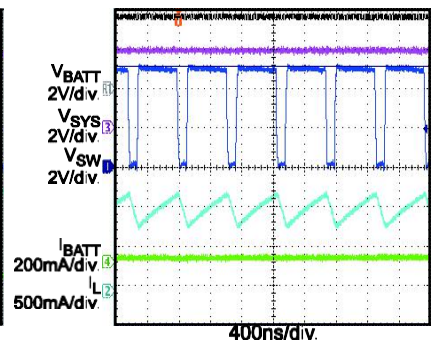
CC Steady State USB3.0 Mode, V_{BATT} = 3.8V I_{SYS} = 1.5A
