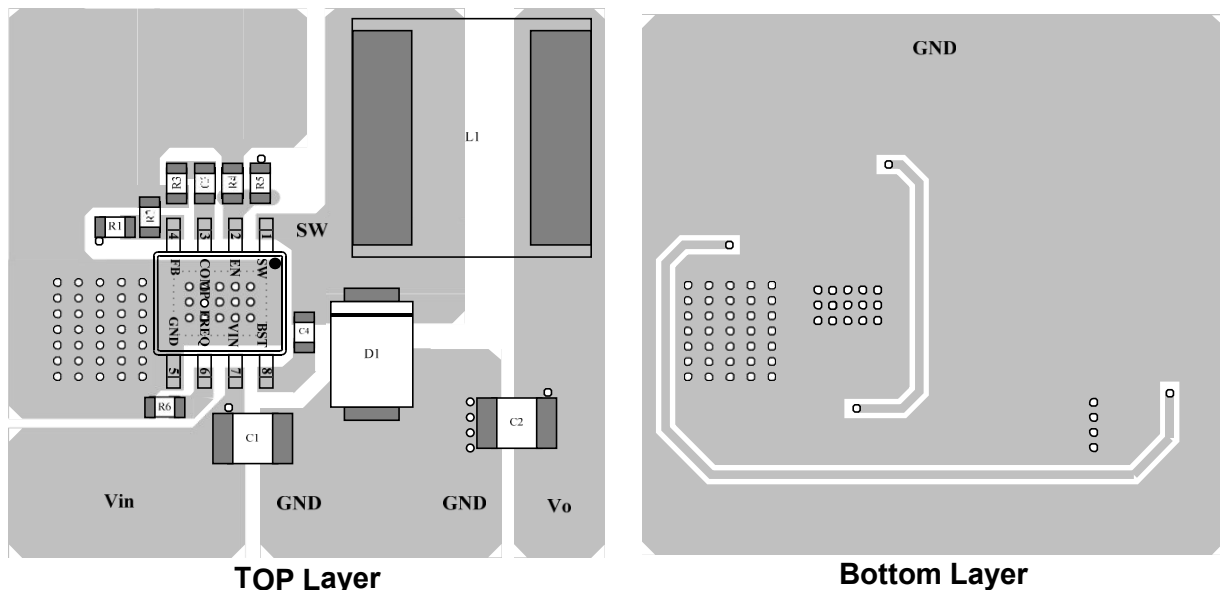
Figure 5—MP2467 Typical Application Circuit and PCB Layout Guide
