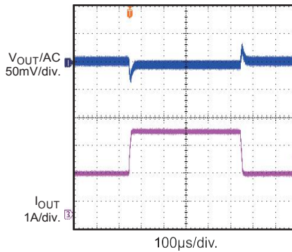
Load Transient Response I_{OUT} = 1.5A to 3A
