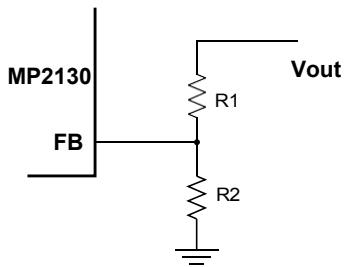
Figure 2— Feedback Network
