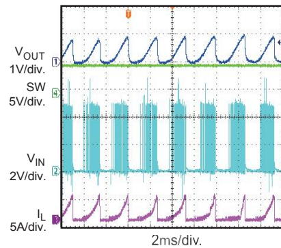
Short Circuit
