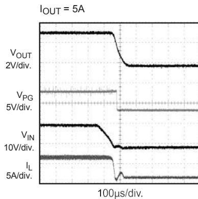
Power Down
