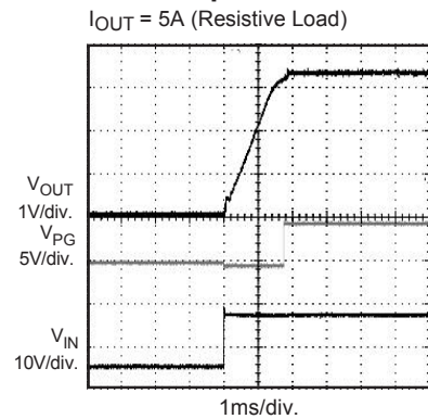
Power Up
