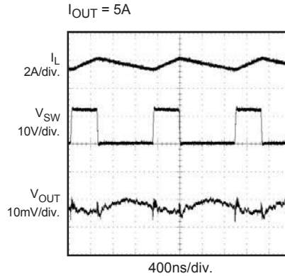
Output Ripple
