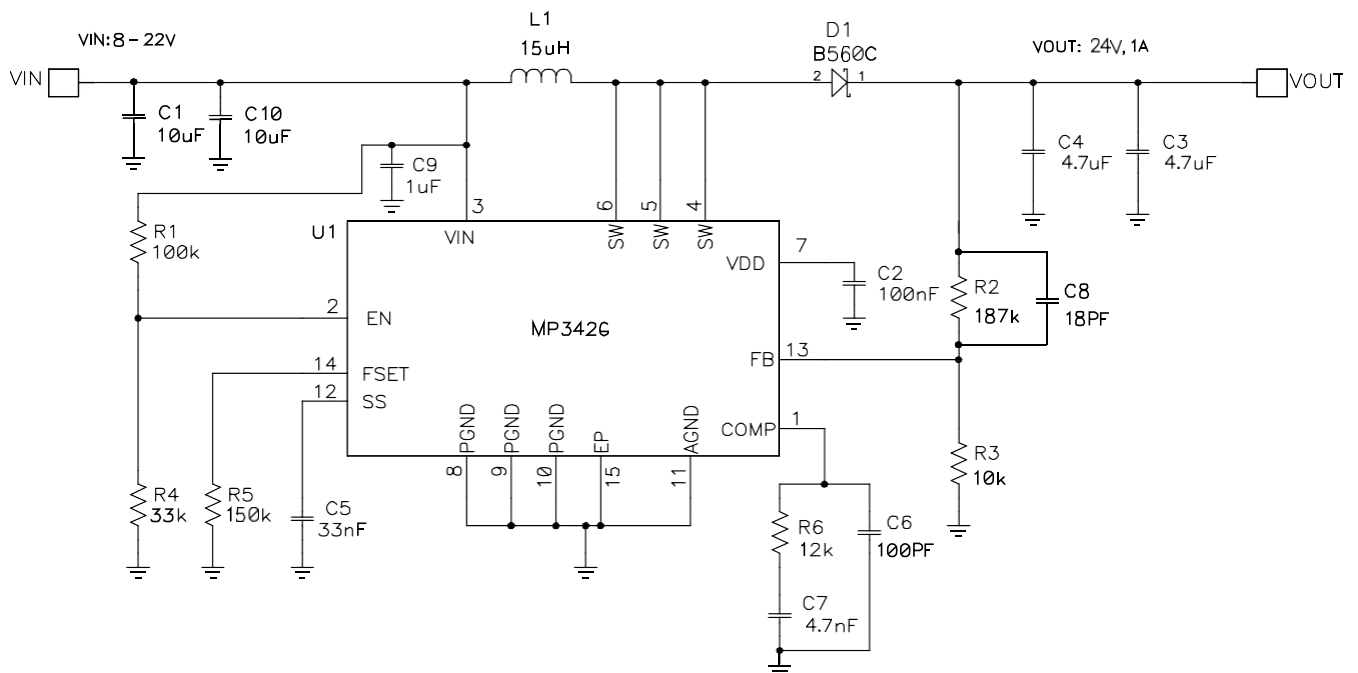
Figure 5: Typical Application Schematic—24V Output
