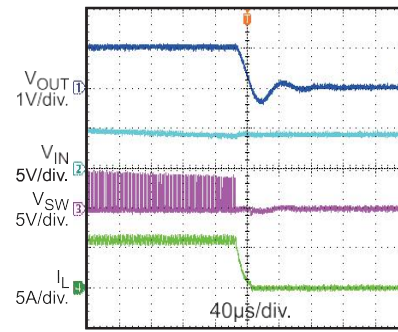
Shutdown Through V_{IN} I_{OUT} = 6A
