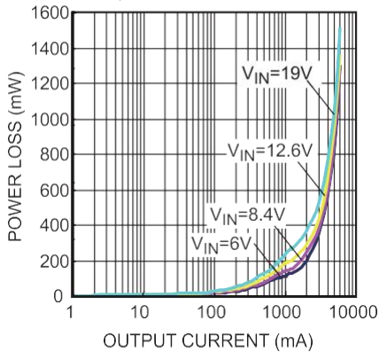
Power Loss
