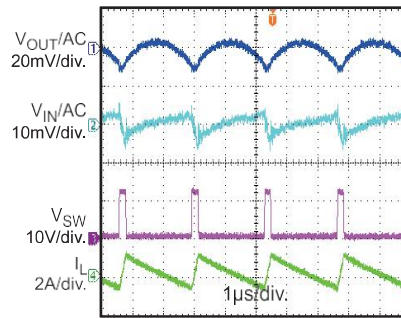
Input/Output Voltage Ripple I_{OUT} = 0A , PWM Mode
