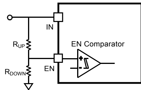
Figure 9: Adjustable UVLO
