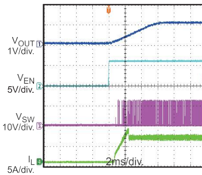
Start Up Through EN I_{OUT} = 6A
