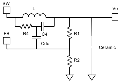
Figure12: Simplified Circuit of Ceramic Capacitor with DC blocking capacitor Input Capacitor
