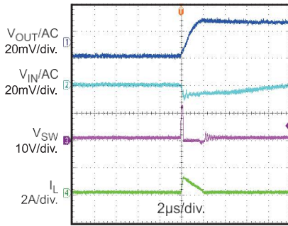
Input/Output Voltage Ripple I_{OUT} = 0A
