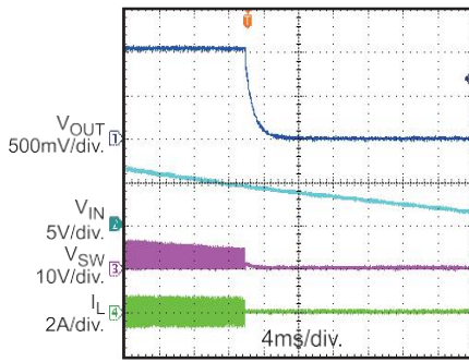
Shutdown Through V_{IN} I_{OUT} = 0A , PWM Mode
