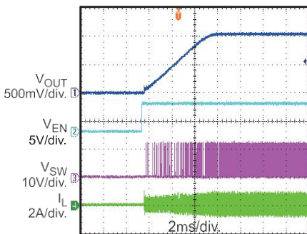
Start Up through EN I_{OUT} = 0A , PWM Mode
