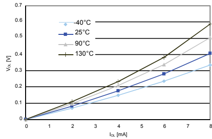
Figure 31. Typical V_{OL} @ V_{DD} = 1.8 V (high sink ports)
