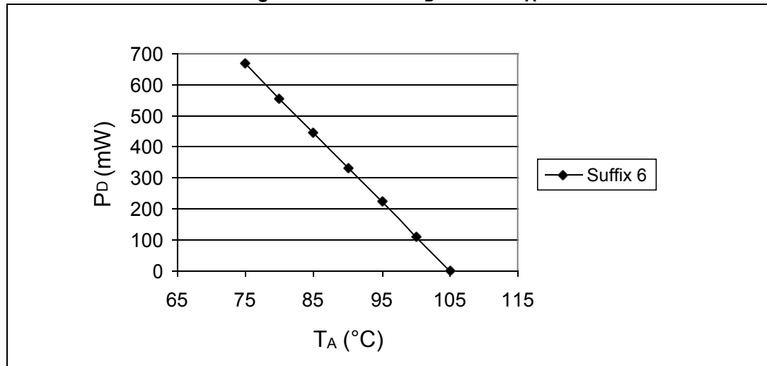
Figure 52. LQFP64 P_D max vs. T_A
