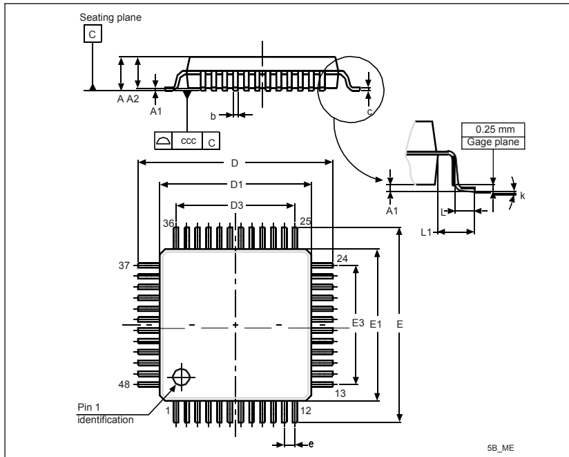
Figure 44. LQFP48, 48-pin low-profile quad flat package outline (1)
