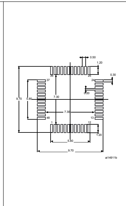
Figure 45. Recommended footprint (1)(2)
