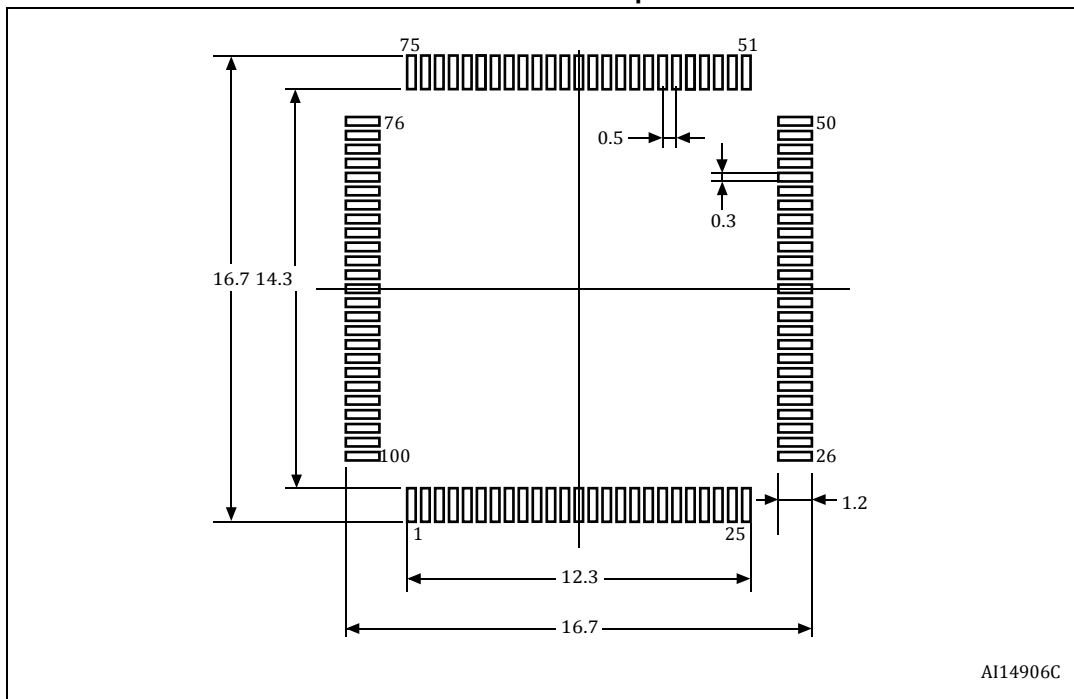
Figure 42. LQPF - 100-pin, 14 x 14 mm low-profile quad flat package recommended footprint
