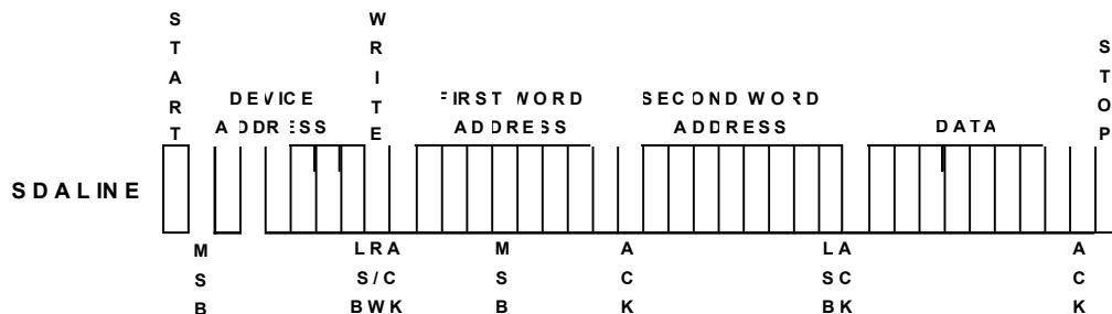
Figure 5: Byte Write
