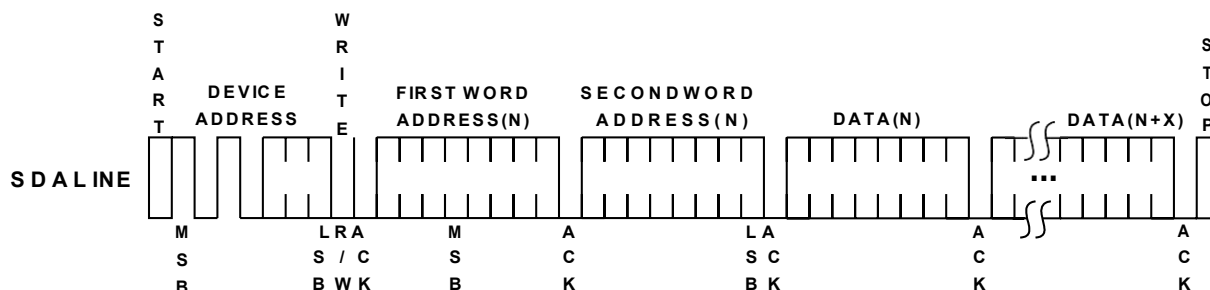
Figure 6: Page Write
