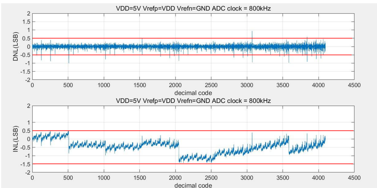
图 18-1 DNL and INL @ V_{REFP} = V_{DD} = 5\text{V} , F_{ADCLK} = 800\text{kHz}
