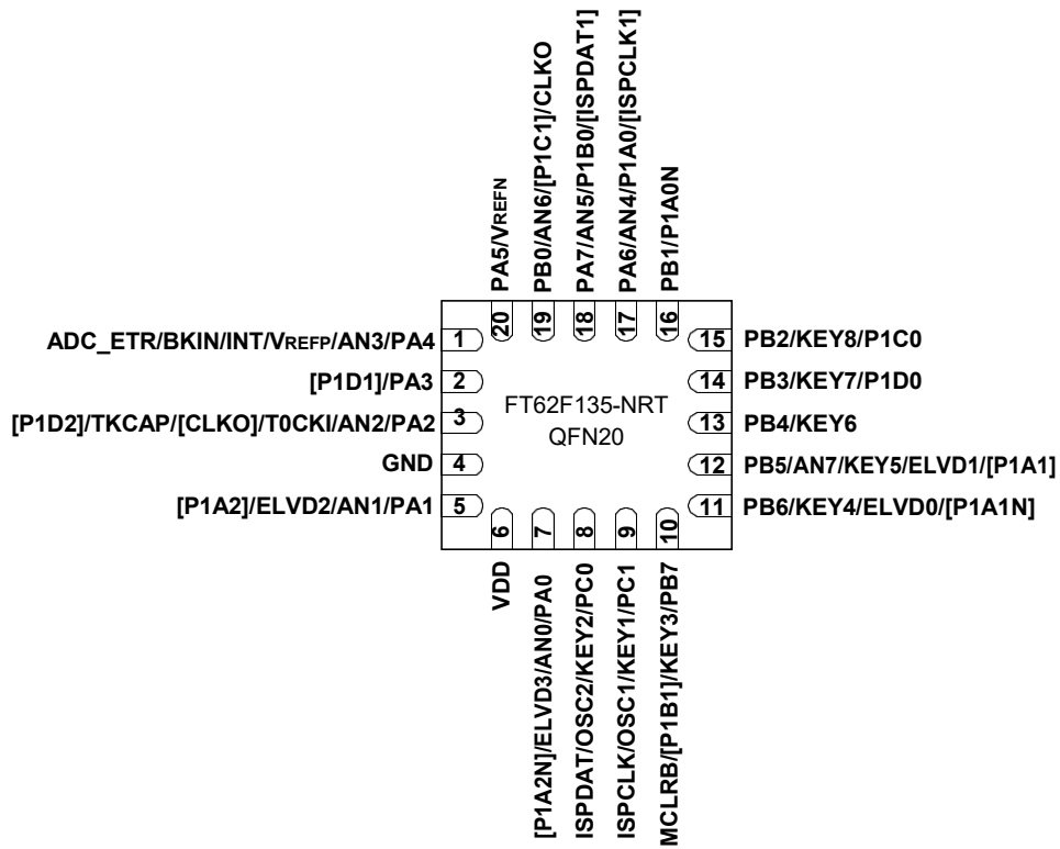
图 1-7 QFN20 2
