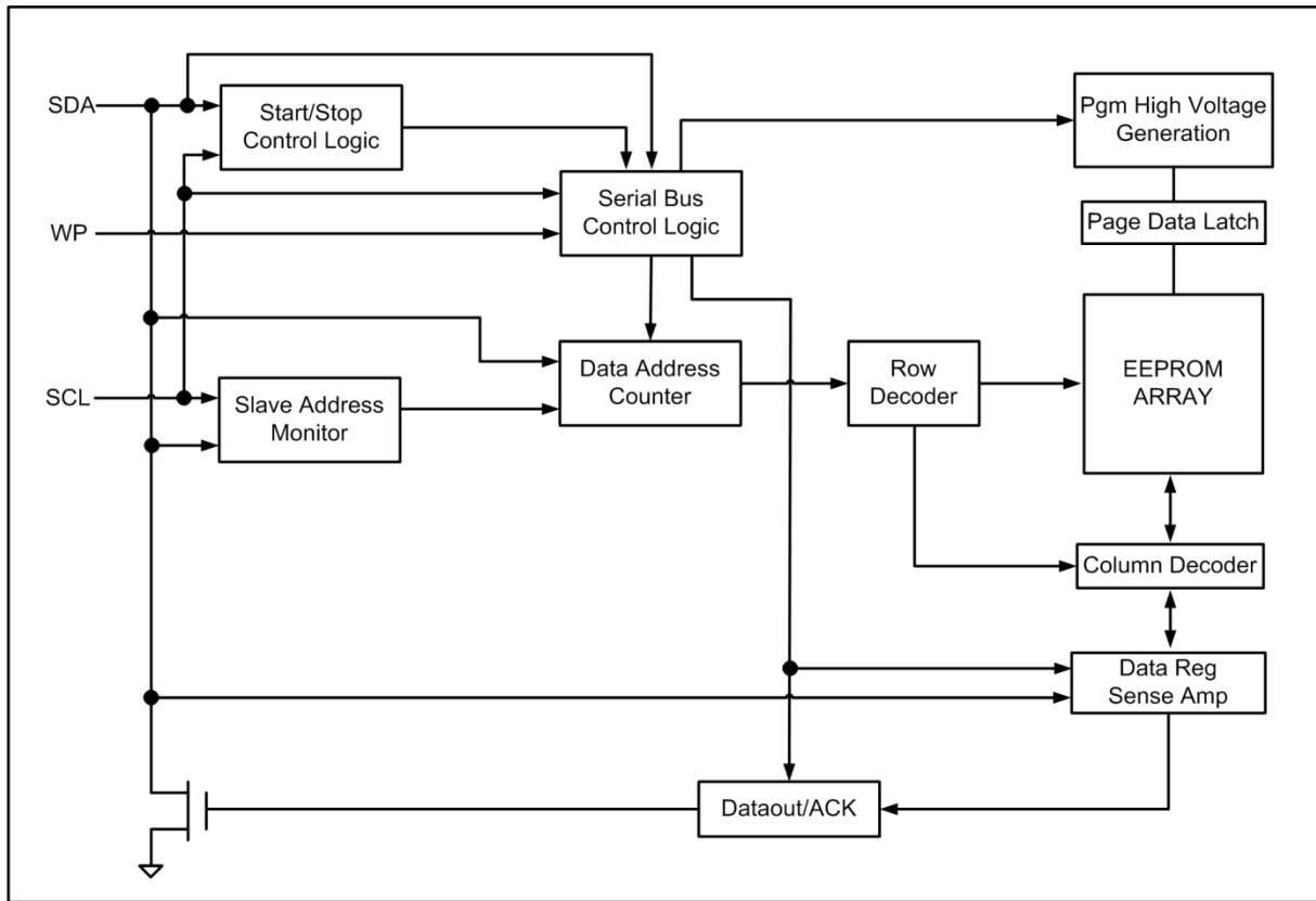
Figure 2: Block Diagram
